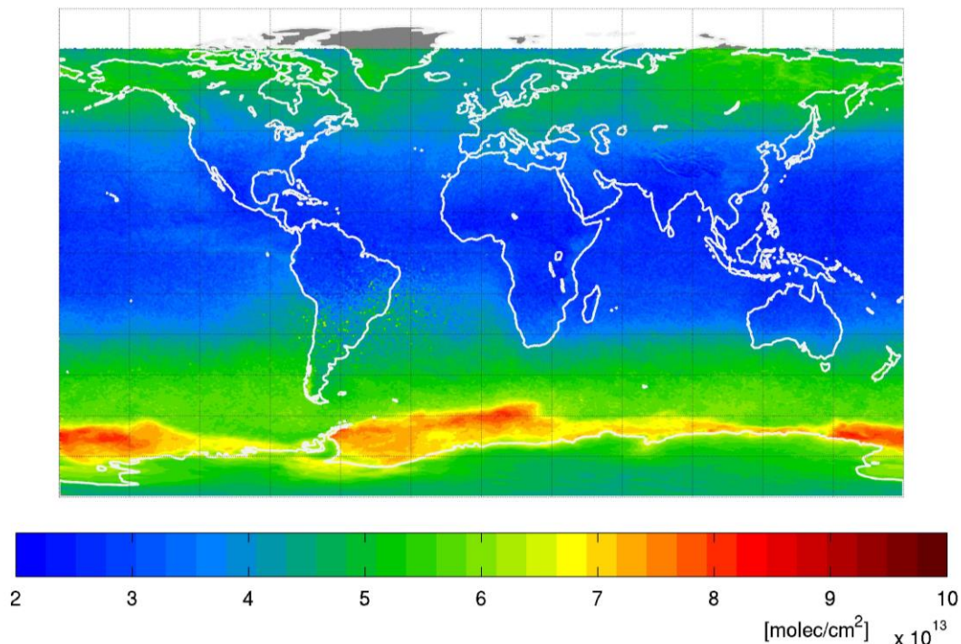
Figure 1. Monthly averaged of GOME-2A BrO vertical columns retrieved for October 2007 (using the baseline settings given in Table 1).
