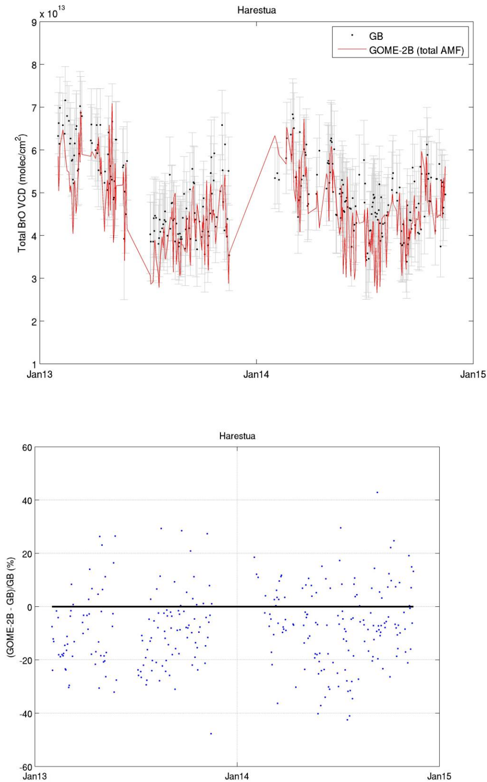
Figure 15. (upper plot) Comparison of BrO total columns retrieved from GOME-2B and ground-based UV-visible measurements at the Harestua station (data originators: F. Hendrick), (lower plot) relative difference between GOME-2B and ground-based BrO columns.
