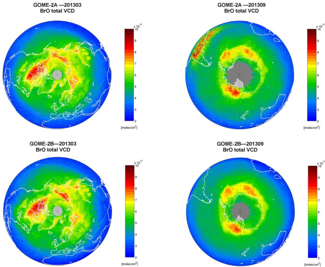
Figure 6. Monthly averages of GOME-2A (top) and GOME-2B (bottom) total BrO vertical columns in polar spring (2013) for the Northern Hemisphere (March: left plots) and the Southern Hemisphere (September: right plots). Only data corresponding to solar zenith angles lower than 80^\circ are used.
