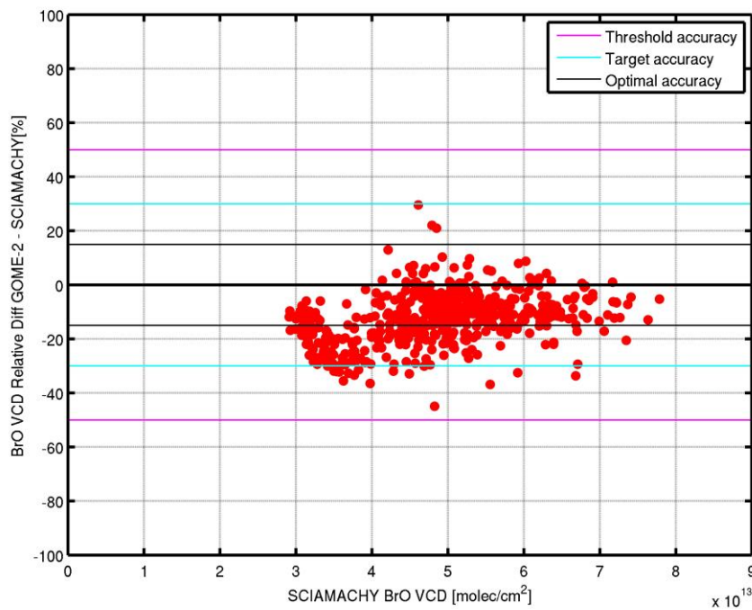
Figure 10. Relative difference in BrO VCD between GOME-2A and SCIAMACHY plotted as a function of SCIAMACHY BrO VCD.
