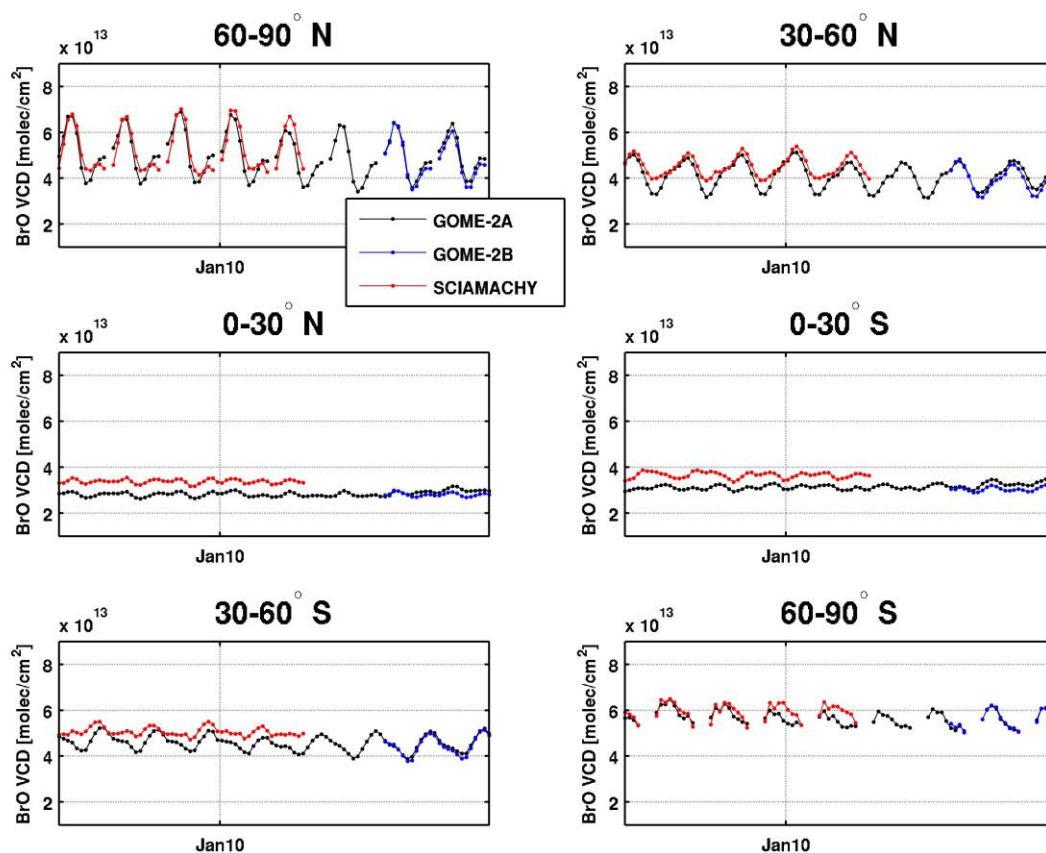
Figure 12. Time-series of total BrO vertical columns from GOME-2A, GOME-2B and SCIAMACHY observations (2007-2014) for different latitudinal bands (monthly zonal averages). Only data corresponding to solar zenith angles lower than 80^\circ are shown.
