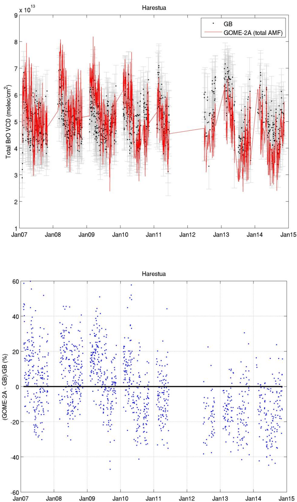
Figure 13. (upper plot) Comparison of BrO total columns retrieved from GOME-2A and ground-based UV-visible measurements at the Harestua station (data originator: F. Hendrick), (lower plot) relative difference between GOME-2A and ground-based BrO columns.
