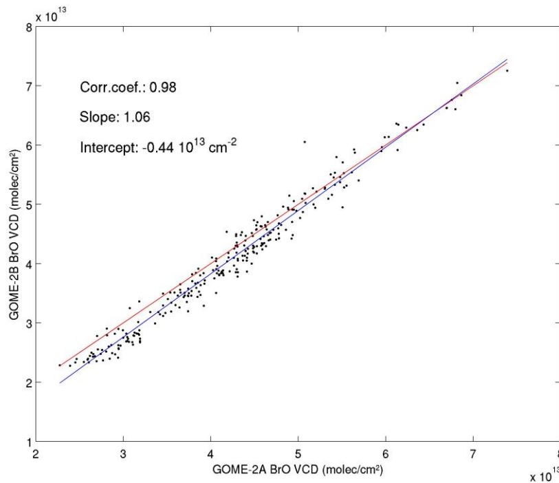
Figure 11. Correlation between BrO VCD retrieved from GOME-2A and GOME-2B. The blue line is the linear regression line (slope: 1.06, intercept: -4.4 \cdot 10^{12} molec/cm 2 ; correlation coefficient: 0.98). The red line represents the reference line of slope equal to unity.
