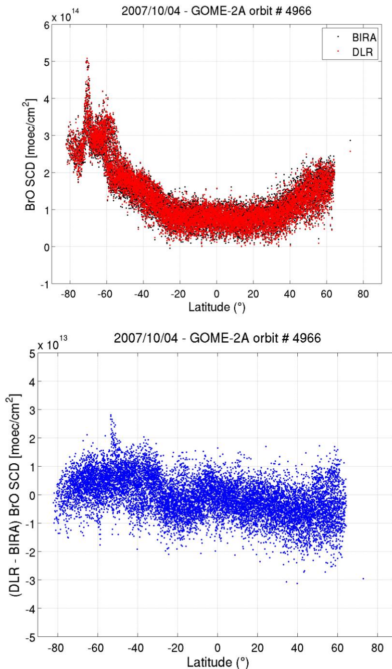
Figure 3. GOME-2A: Comparison of BrO slant columns retrieved from GDP 4.8 and from the BIRA-IASB scientific algorithm. The lower plot corresponds to the difference between GDP 4.8 and BIRA-IASB BrO SCDs. DOAS settings were synchronized according to Table 1.
