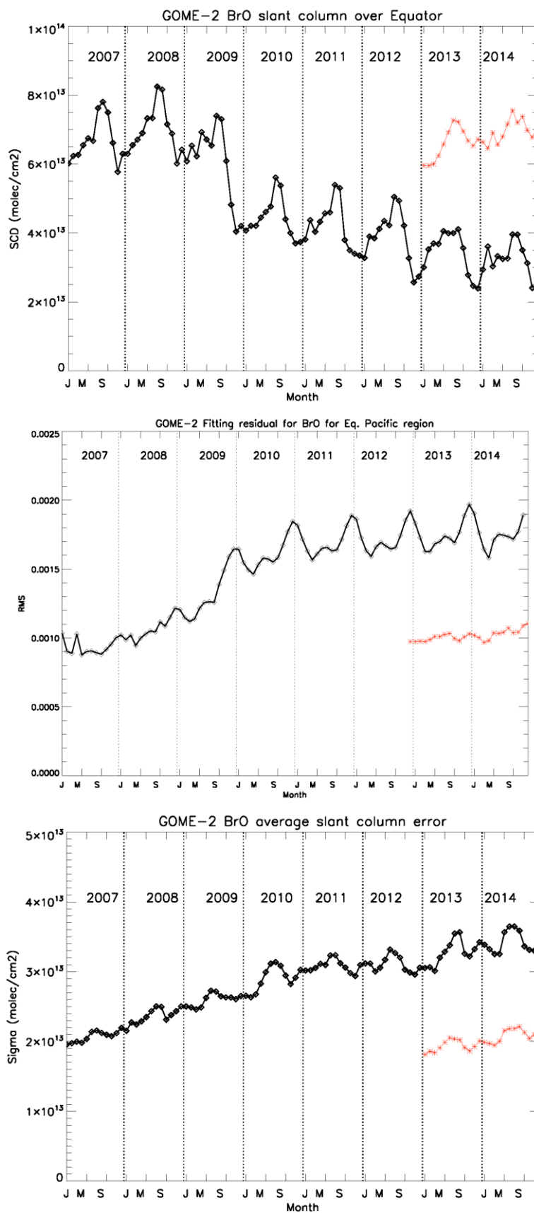
Figure 2. Average BrO slant columns (top), DOAS fitting residuals (middle) and slant column error (bottom) in the equatorial Pacific for GOME-2A (black) and GOME-2B (red).
