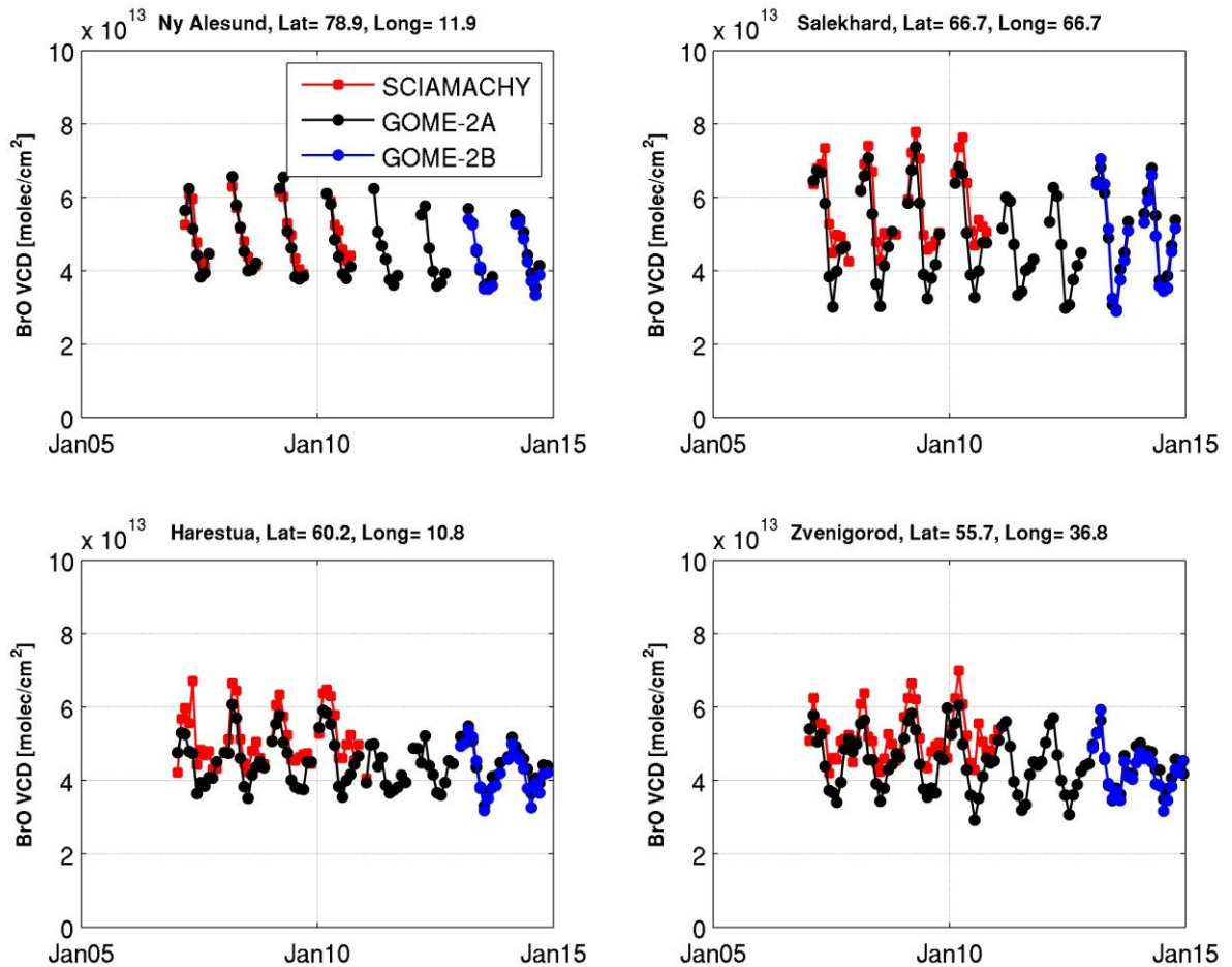
Figure 8. Comparison of time-series of monthly averaged BrO vertical columns retrieved from SCIAMACHY, GOME-2A and GOME-2B over the January 2007- December 2014 period, at a number of ground-based sites.
