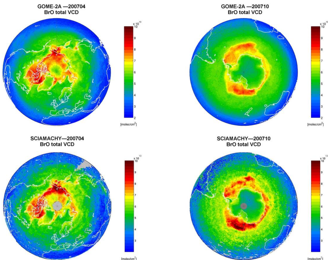
Figure 5. Monthly averages of GOME-2A (top) and SCIAMACHY (bottom) total BrO vertical columns in polar spring (2007) for the Northern Hemisphere (April: left plots) and the Southern Hemisphere (October: right plots). Only data corresponding to solar zenith angles lower than 80^\circ are used.
