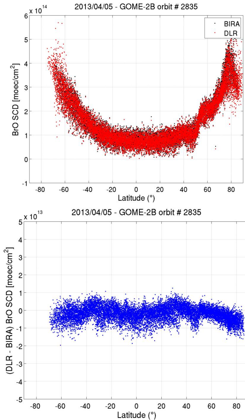
Figure 4. GOME-2B: Comparison of BrO slant columns retrieved from GDP 4.8 and from the BIRA-IASB scientific algorithm. The lower plot corresponds to the difference between GDP 4.8 and BIRA-IASB BrO SCDs. DOAS settings were synchronized according to Table 1.
