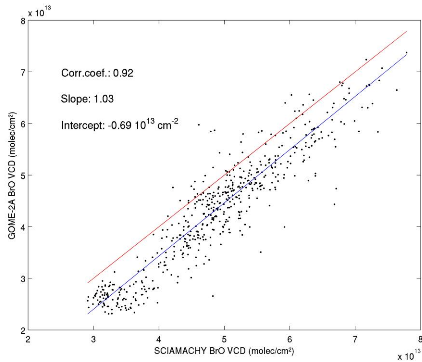
Figure 9. Correlation between BrO VCD retrieved from GOME-2A and SCIAMACHY. The blue line is the linear regression line (slope: 1.03, intercept: -6.9 10 12 molec/cm 2 ; correlation coefficient: 0.92). The red line represents the reference line of slope equal to unity.
