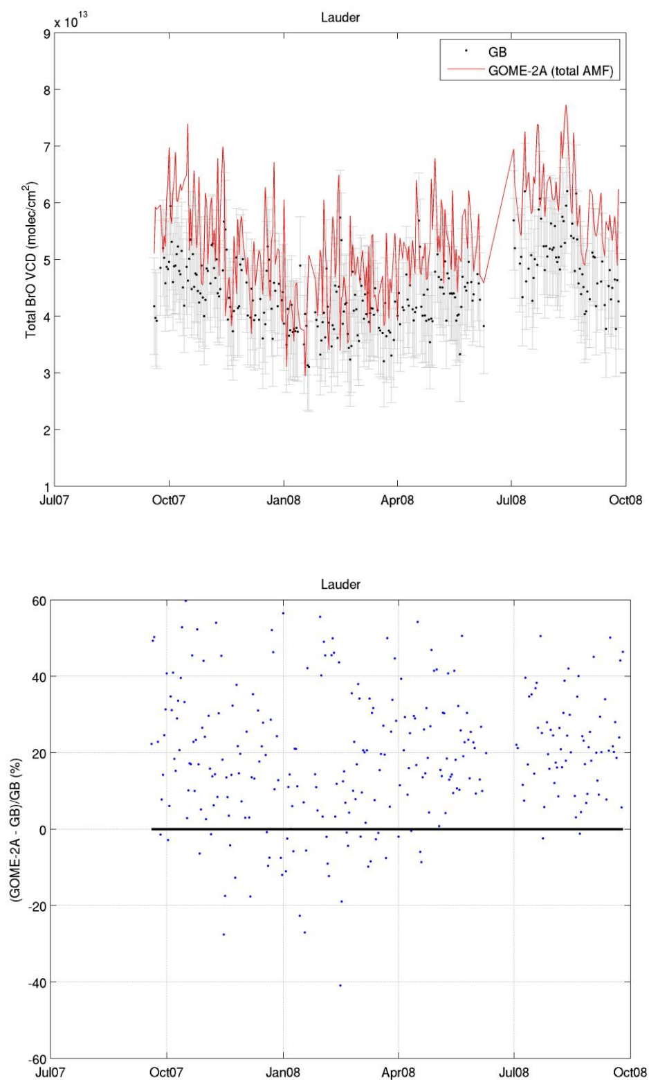
Figure 14. (upper plot) Comparison of BrO total columns retrieved from GOME-2A and ground-based UV-visible measurements at the Lauder station (data originators: P. Johnston and F. Hendrick), (lower plot) relative difference between GOME-2A and ground-based BrO columns.
